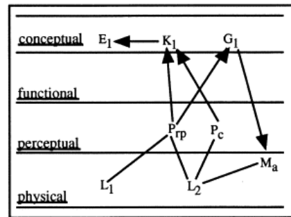
Fig. 5. Relations among design actions for a segment Gero 14 , pp. 471
